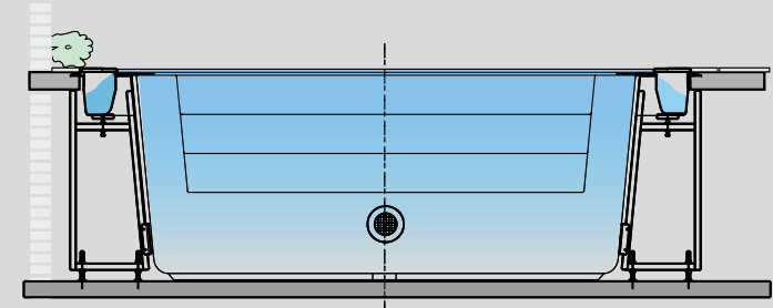
Self-supporting installation with overflow channel: Steel wall braces.
